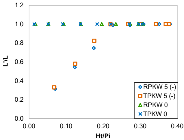
Fig. 8. \frac{L'}{L} ratio versus \frac{H}{P_i} ratio in the sloped and non-sloped rectangular and trapezoidal PKWs.
