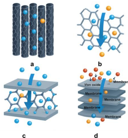
Fig. 3. Schematic illustrations of selected nanomembranes used in wastewater treatment. The illustrations demonstrate (a) carbon nanotube (CNT) channels showing water passing through vertically aligned channels while rejecting larger contaminants; (b) hexagonal boron nitride (h-BN) membranes depicting molecular sieving through nanoscale pores; (c) metal-organic framework (MOF) networks designed for heavy metal ion capture; and (d) iron oxide-based systems where magnetic particles assist in adsorption and recovery.
