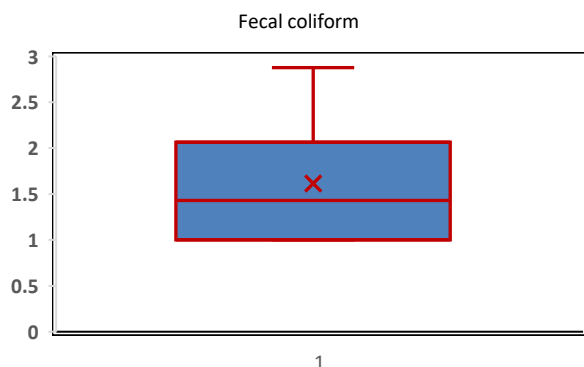
Fig. 3. Boxplot showing monthly logarithmic variations in fecal coliforms (CFU/100 ml) in the Khersan 3 sub-basin.
