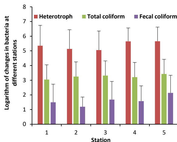
Fig. 5. Stationary logarithmic variations of heterotrophic bacteria, total coliforms, and fecal coliforms (CFU/100 ml) across sampling stations in the Khersan 3 sub-basin (Indicators without letters showed no significant differences).
