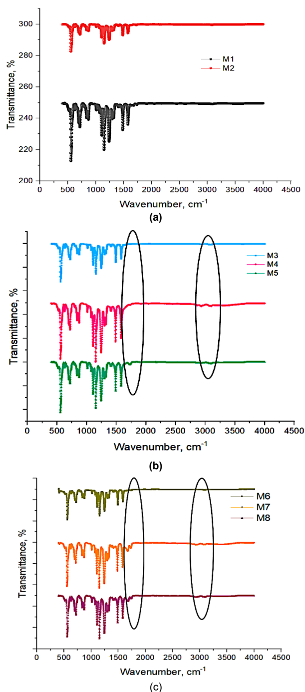
Fig.2. ATR-FTIR spectrum of M1 and M2 (a); M3, M4, and M5 (b); M6, M7, and M8 (c).
