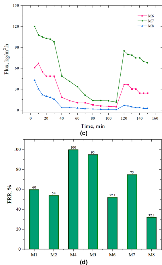
Fig. 4. Three-step filtration performance of M1 and M2 (a); M3, M4, and M5 (b); M6, M7, and M8 (c); and FRR of the fabricated membranes (d).
