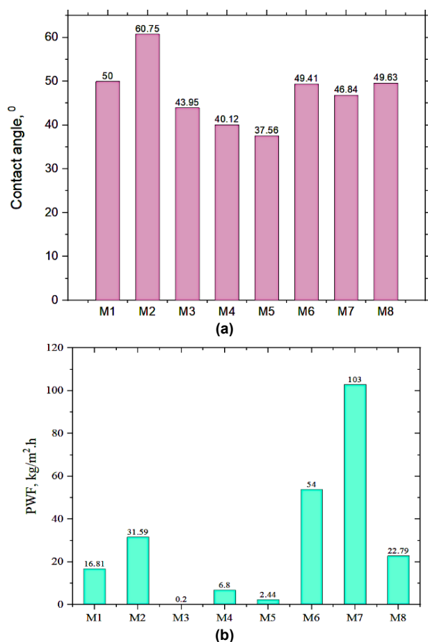
Fig.3. Contact angles (a) and PWFs (b) of the fabricated membranes.
