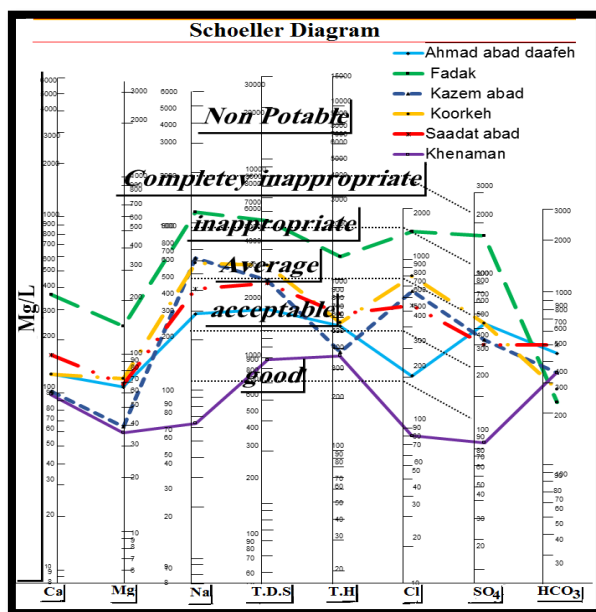
Fig. 7. Water quality of the studied aqueducts for drinking water consumption based on the Schoeller diagram.
