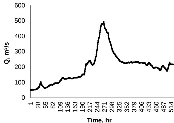
Fig. 9. Observed run off in Faraman station on 03/04/2019.
