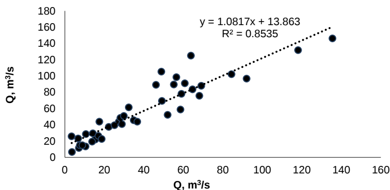
Fig. 5. IMF regression in Faraman and Pole-kohne stations (up), maximum daily flood between Doab mereg and Khersabad stations (Down).
