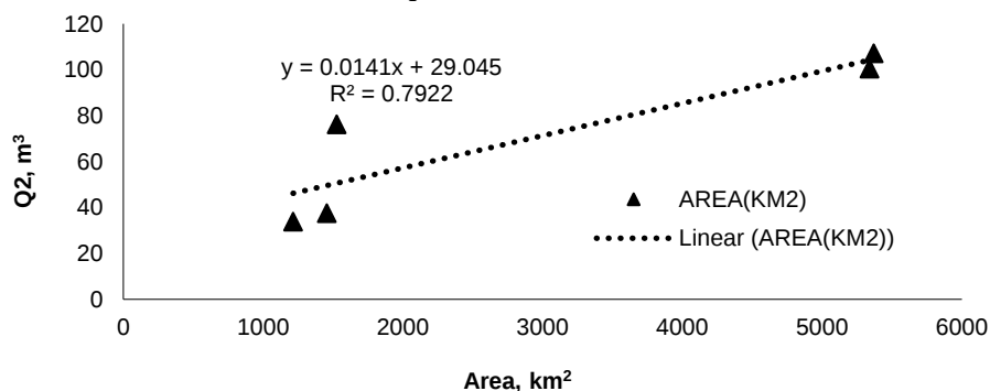
Fig. 7. Linear regression between AREA.
