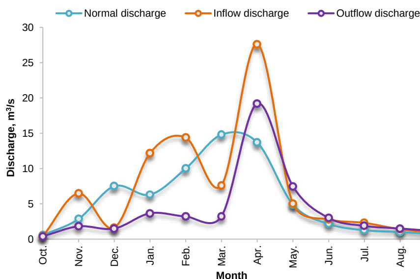
Fig. 10. Average monthly discharge curve of the Balaroud river during the third water year (September 23, 2022 - September 22, 2023) compared to normal discharge.
