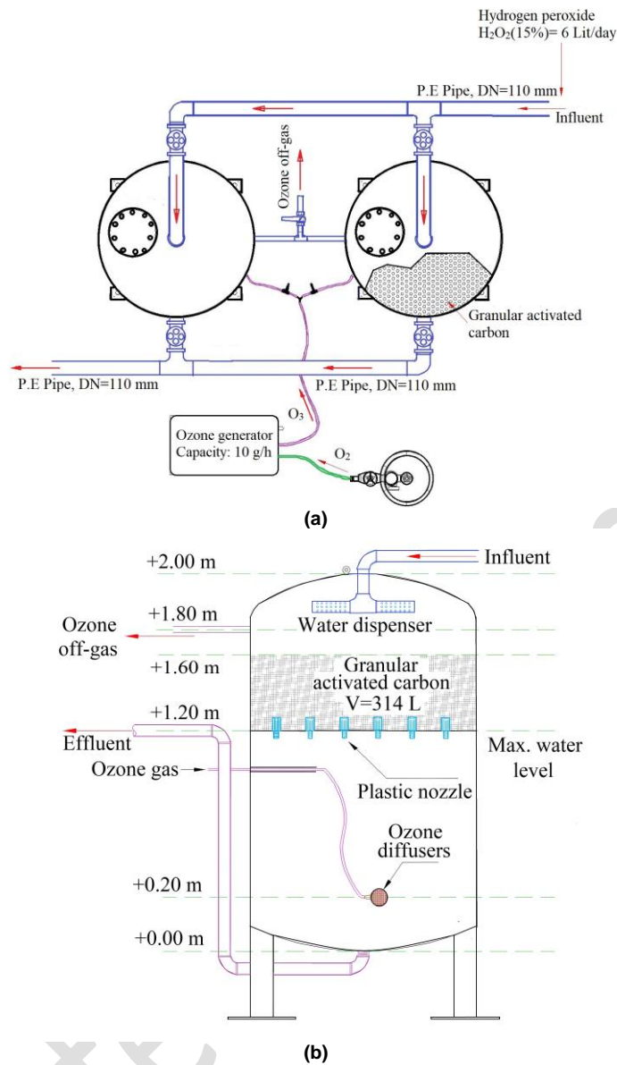
Fig. 1. The designed AOP reactor (a) plans for the reactors; (b), cross section of one of the reactors.
