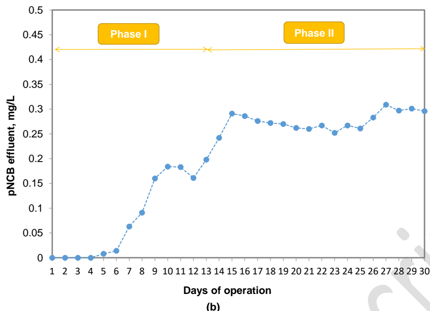
Fig. 2. Variation of pNCB concentration for both influent (a) and effluent (b) with operation time.
