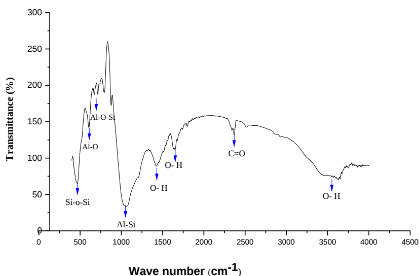
Fig. 3. FTIR spectra of natural Sabzevar zeolite.
