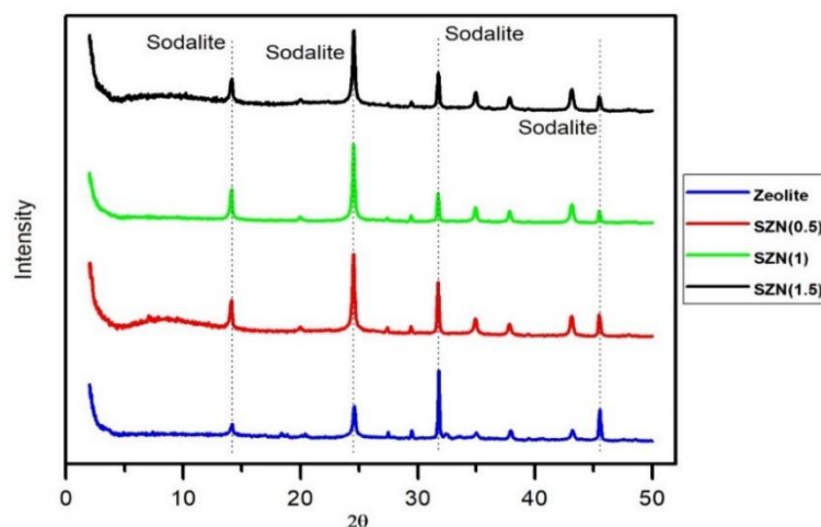
Fig. 17. XRD pattern of SZN, and Zeolite with different ratios (Mahmoodi and Saffar-Dastgerdi, 2019).
