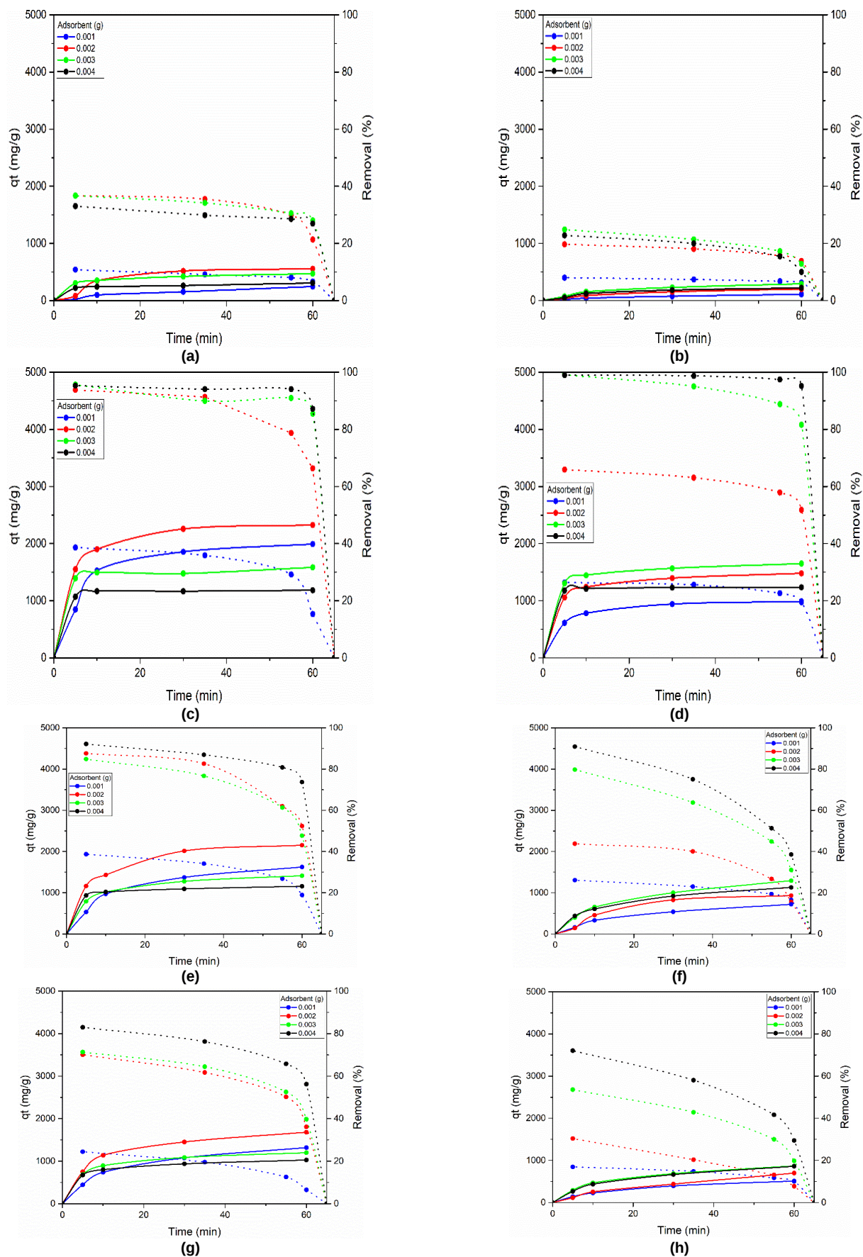
Fig. 22. Effect of adsorbent dose on pollutant removal by Zeolite ,and SZN (Mahmoodi and Saffar-Dastgerdi, 2019).
