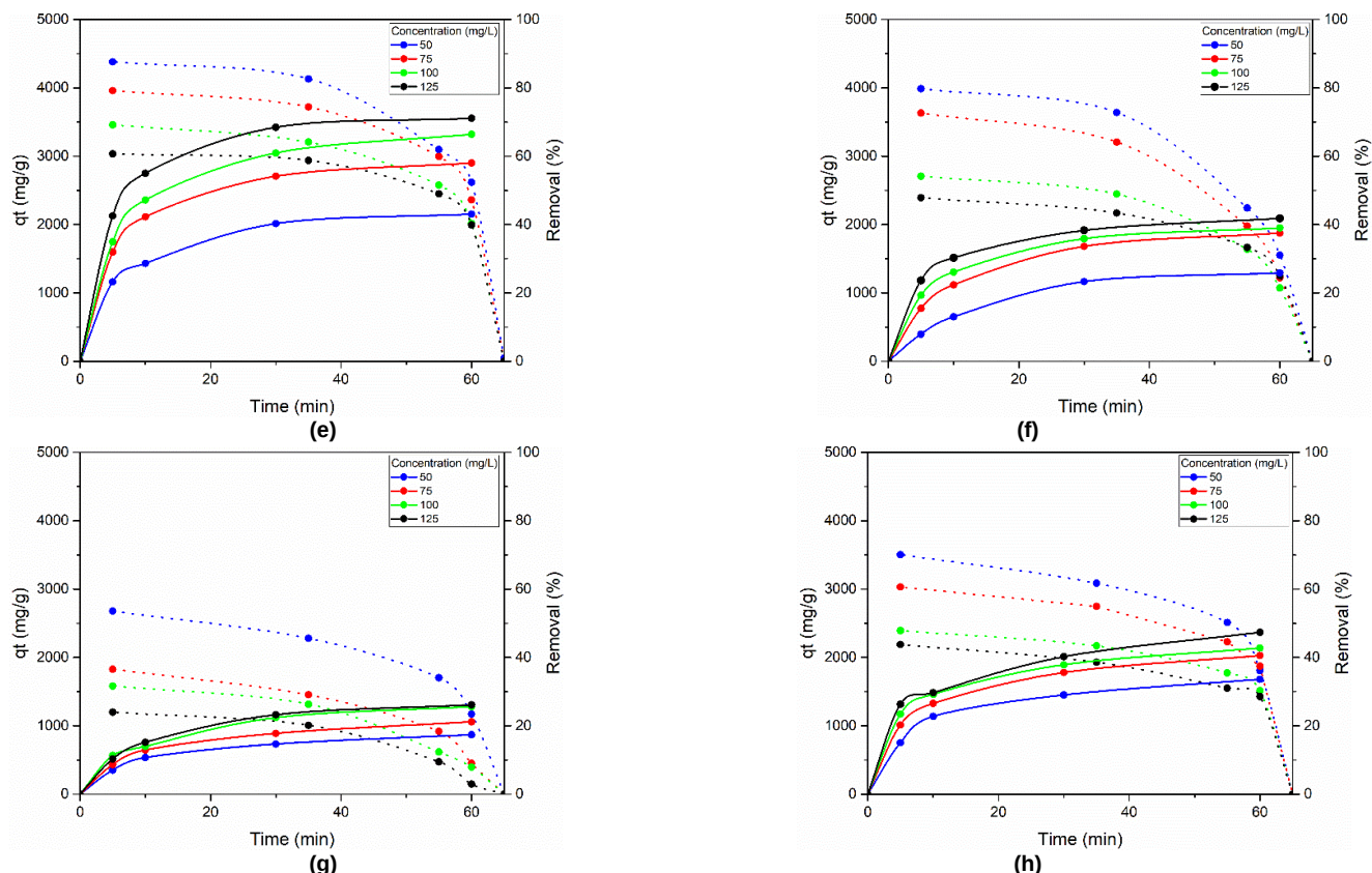
Fig. 23. Effect of initial concentrations on pollutant removal by Zeolite, and SZN (Mahmoodi and Saffar-Dastgerdi, 2019).
