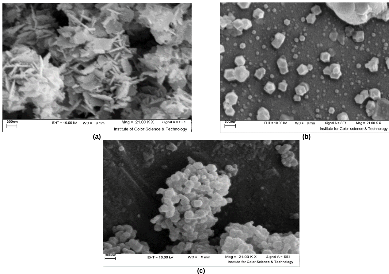
Fig. 16. SEM images of (a) ZnO, (b) ZIF-8, and (c) ZnO-ZIF-8 composite (Mahmoodi et al. , 2021).
