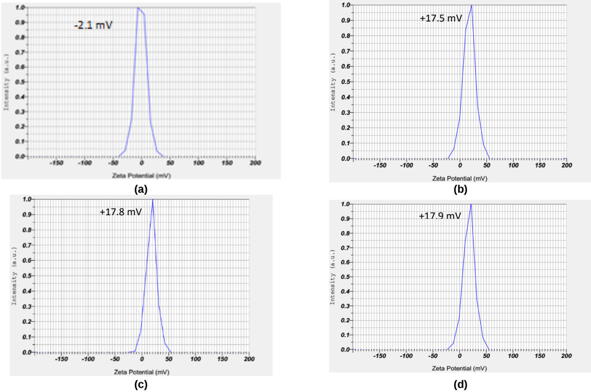
Fig. 19. Zeta potential graph of (a) zeolite, (b) SZN(0.5), (c) SZN(1) and (d) SZN(1.5) (pH= 2.1) (Mahmoodi and Saffar-Dastgerdi, 2019).
