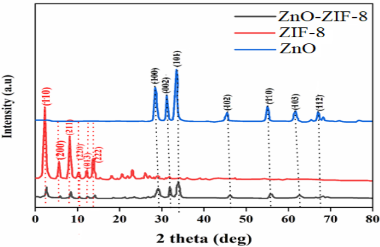
Fig. 18. XRD pattern of ZnO,ZIF-8, and ZnO-ZIF-8 (Mahmoodi et al. , 2021).
