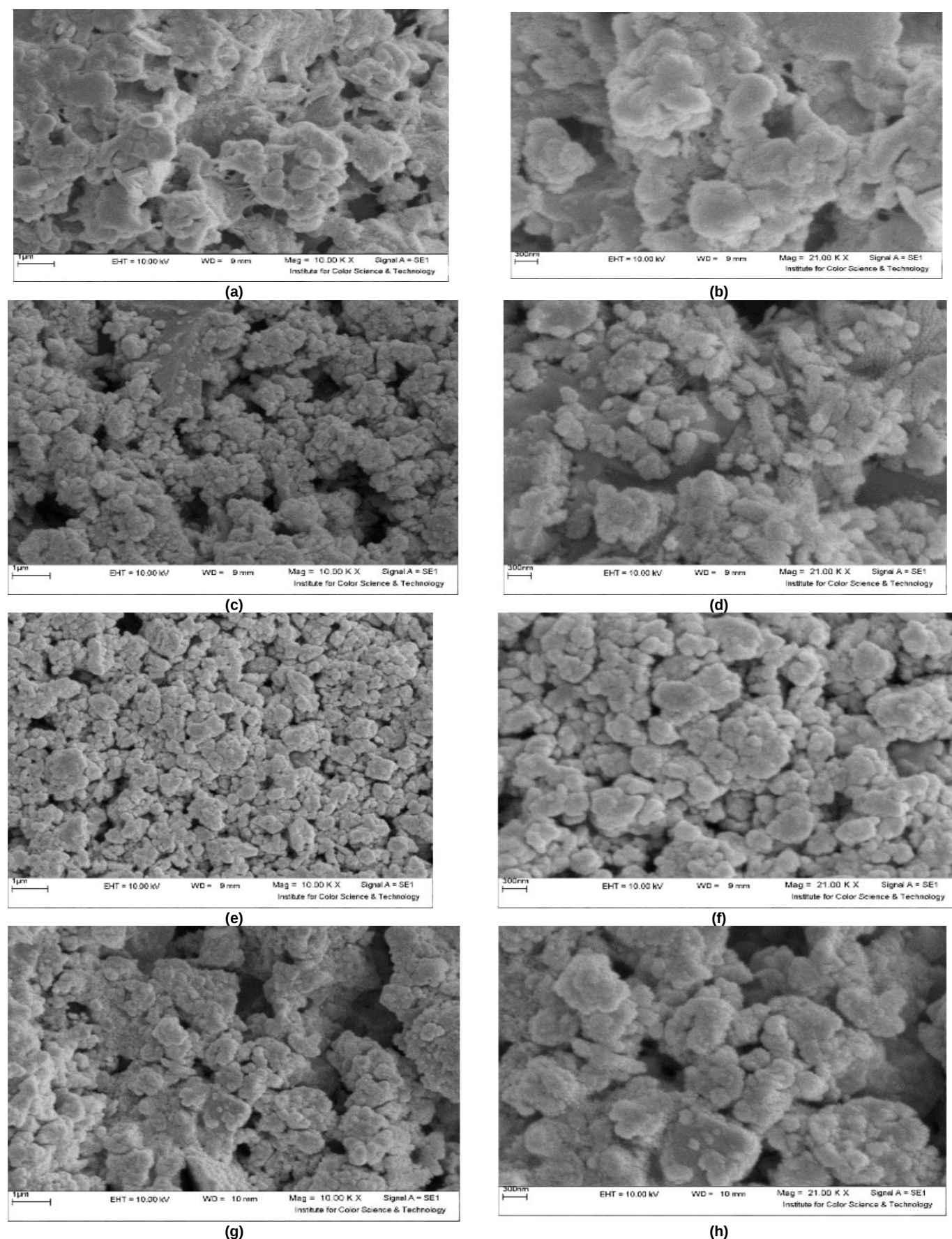
Fig. 15. SEM images of (a,b) zeolite, (c,d) SZN (0.5), (e,f) SZN (1) and (g,h) SZN (1.5) (Mahmoodi and Saffar-Dastgerdi, 2019).
