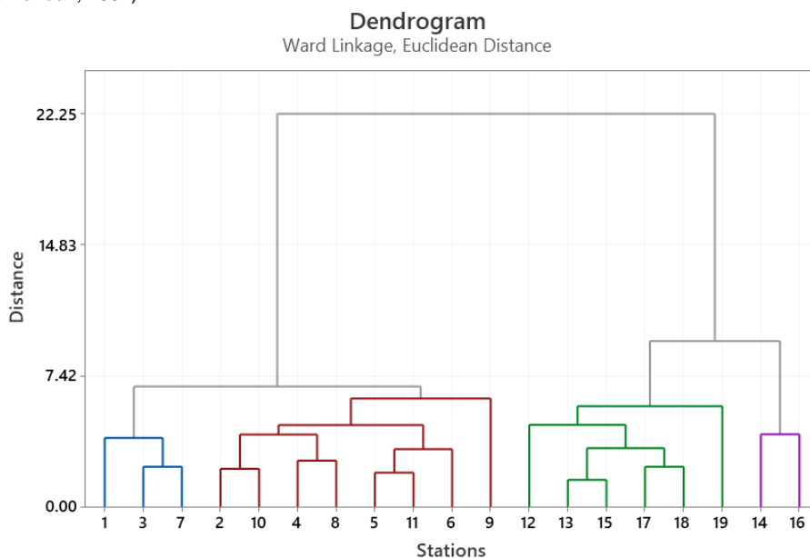
Fig. 2. Cluster diagram of qualitative grouping of the studied stations based on parameters measured in the Aras River, Iran.
