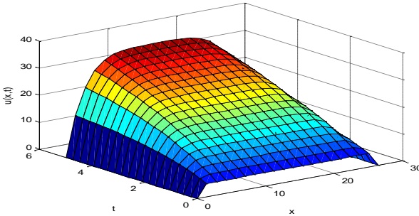
Fig. 6. Concentration of BOD in Scenario two after implying model.
