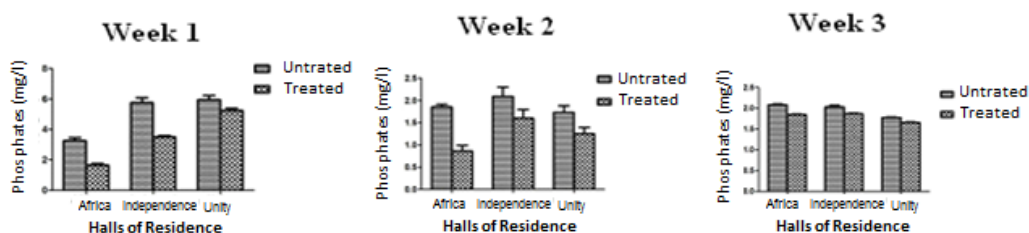
Fig. 8. Phosphates levels for untreated and treated grey water from Africa, Independence and Unity Halls.
