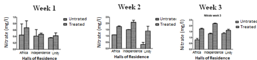
Fig. 7. Nitrate levels for untreated and treated grey water from Africa, Independence and Unity Halls.
